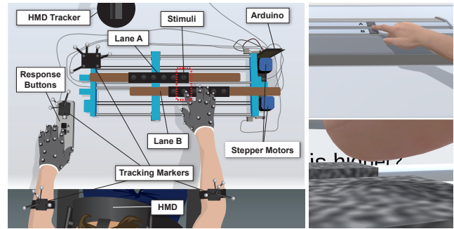
Figure 2: Illustration of the apparatus (l), screenshot of the virtual view (t.r) and close up of the virtual stimuli (b.r.).
